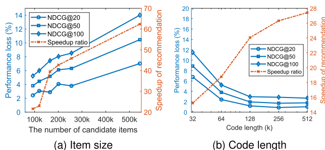
Fig. 9. Sensitive analysis of the two-stage model in the Amazon dataset.
